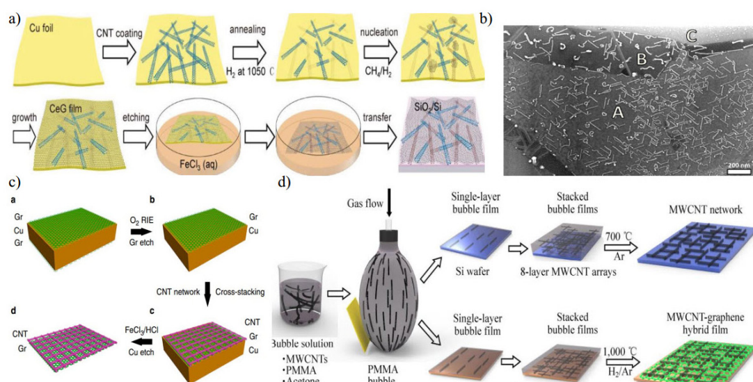
Figure 2. Scheme for CNT-graphene parallel heterostructure. (a) Graphene grown by Chemical Vapor deposition using CNTs as templates [56]. (b) CNTs grown by Chemical Vapor deposition using graphene film as template [57]. (c) Cross-staking CNT networks coated on the graphene film [81]. (d) By blown bubble method [55].
